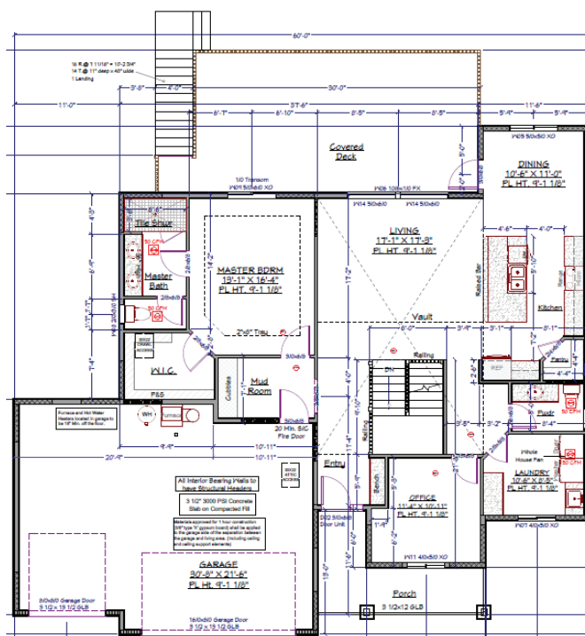
1st Floor
